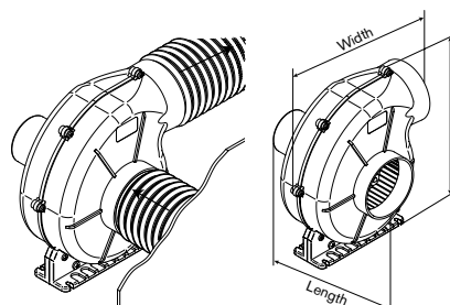
Flex Mount
