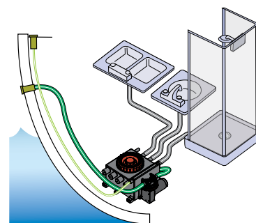
Grey Water Tank with Viking Power 16
